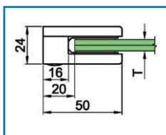
Modell 405 H 40,0 x B 50,0 x T 26,0 mm
