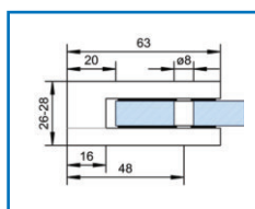
Modell 456 H 45,0 x B 63,0 x T 30,0 mm
